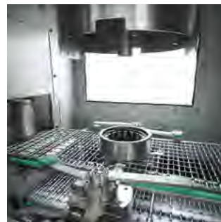
YukonDA Continuous system with lance system for horizontal transport
